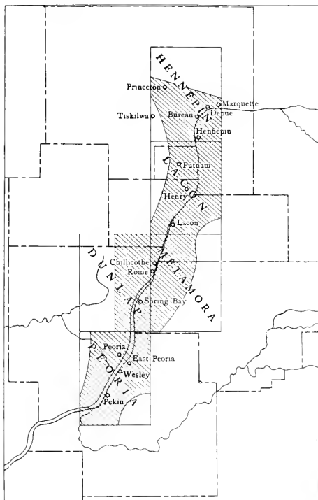
FIG. 1. Index map showing towns, quadrangles, and the area covered by this report.
